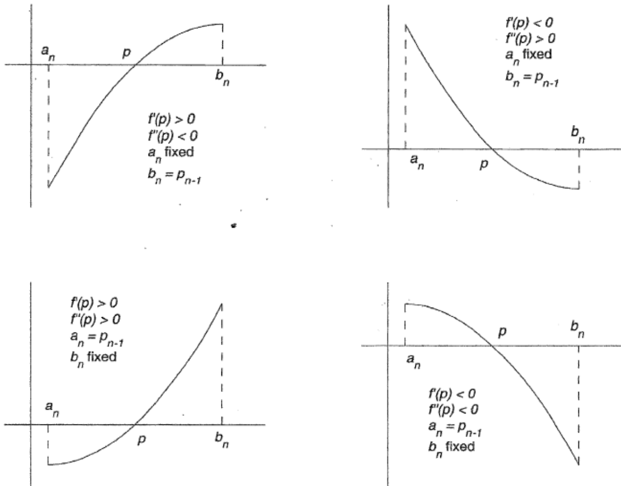
Figure 2.5 Eventual configurations for the method of false position.
